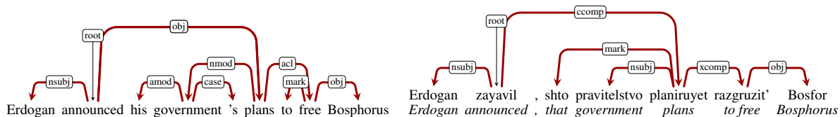
Figure 2: A pair of sentences from the En-Ru PUD corpus that exemplifies a clausal complement ( ccomp headed by planiruyet in the Russian sentence on the right) that is aligned with a nominal complement of the verb of speech ( obj headed by plans in the English sentence on the left).
