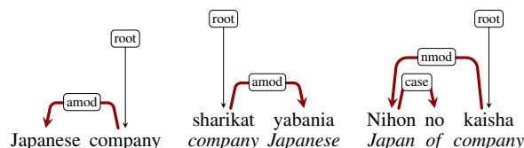
Figure 1: A UD parse of the English phrase Japanese company (left) and of its translations to Arabic (middle) and Japanese (right). Word order aside, the UD tree of the Arabic translation is identical to the English one while that of the Japanese translation is different. The amod edge in this phrase is stable in translation to Arabic but unstable in translation to Japanese.
