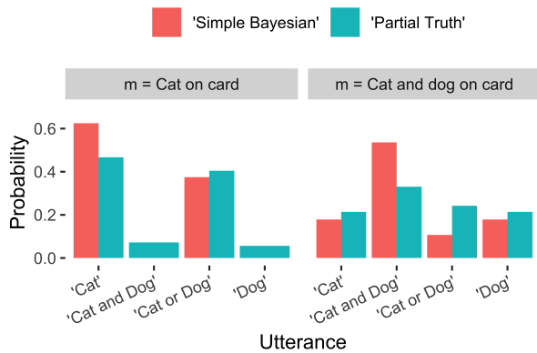
Figure 2: Simulated S_1 production probabilities.
