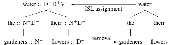
Figure 2: Feature assignment as a transduction problem between a feature-annotated MG dependency tree (left) and its feature-free counterpart (right)
