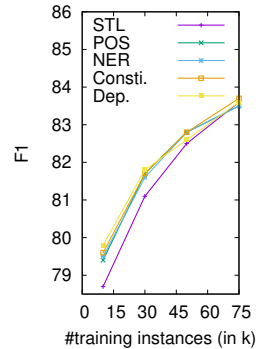
Figure 3: MTL Performance of SRL wrt. the data size.
