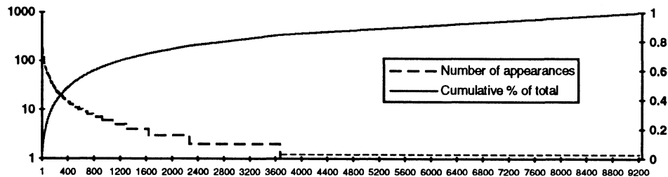
Figure 3 A relatively small number of distinct candidates account for a large number of potentially ambiguous partitions. The most frequent candidate appears 365 times; the top 452 account for half of the total in the text, and about 5,500 appear just once. This strongly Zipfian distribution implies that while it is impossible to anticipate all ambiguous partitions, dealing with the most common is a worthwhile investment of time.
