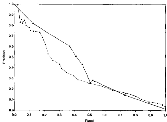
Figure 5: Precision-recall graph comparing our method using RIPPER (solid line with squares) versus TF*IDF (dotted line with triangles).
