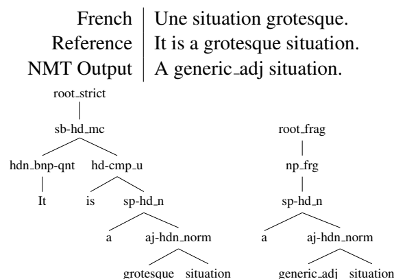
Figure 1: A test set source-reference pair and the NMT translation. Below are parser derivations in the ERG of both the reference and NMT translation. The ERG is described in §2. Non-syntactic rules have been omitted. The NMT model is trained and tested only on sentence pairs where the reference is parseable by the ERG. The NMT translation may not always be parseable. Analysis on model output parseability in §4.1.
