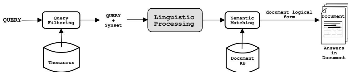
Figure 2: Schematic representation of the core QA engine
