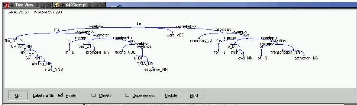
Figure 5: Dependency Tree output of the SWI Prolog graphical implementation of the parser
