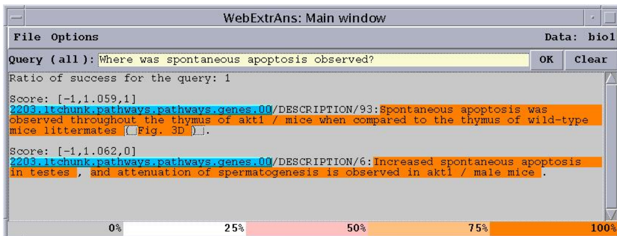
Figure 3: Example of interaction with the system
