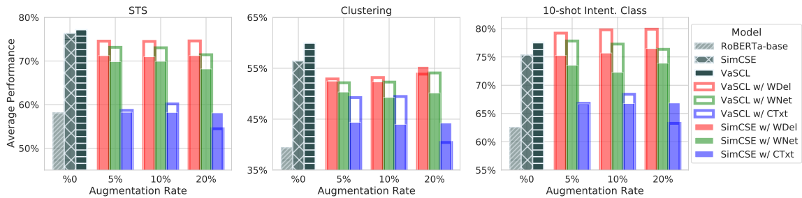
(a) Virtual augmentation vs. explicit augmentation. For each downstream task, we report the mean performance averaged over all its subtasks. The explicit augmentations are evaluated using SimCSE (dropout) for training, i.e. , "SimCSE w/ {WDel/WNet/CTxt}".
