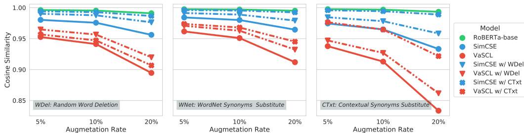
(b) Cosine similarity between each original training example and its augmentation evaluated on the representation spaces of different models. From left to right, the augmentations are obtained via WDel , WNet , and CTxt . Each point is averaged over 20,000 randomly sampled training examples and their augmentations. We exclude "SimCSE w/ WNet" and "VaSCL w/ WNet" for better visualization. Please refer to Figure 4 in Appendix for the full plot.
