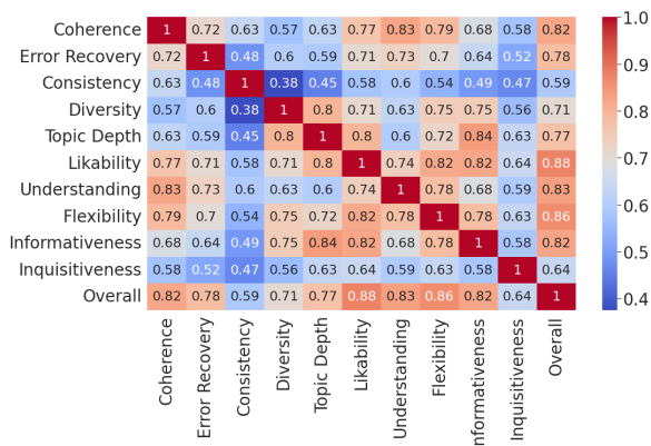
Figure 1: Spearman correlations of dimension pairs on FED.
