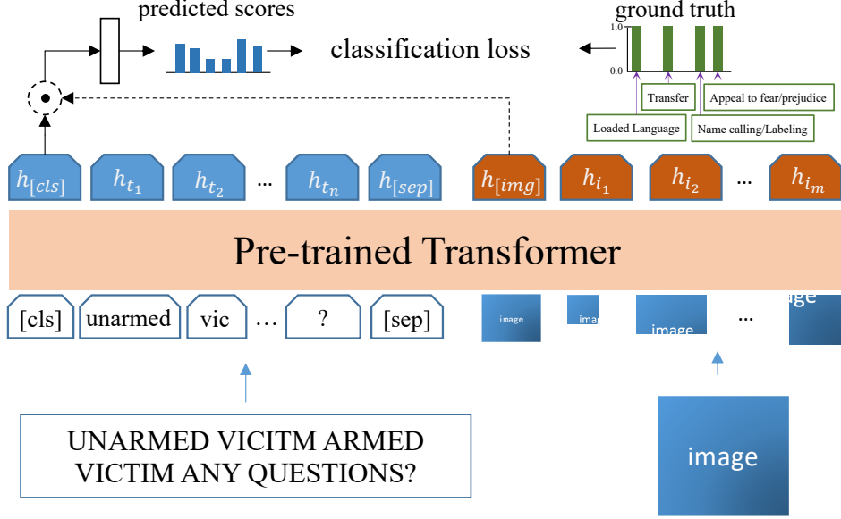
Figure 1: A unified framework used for the multimodal classification task.
