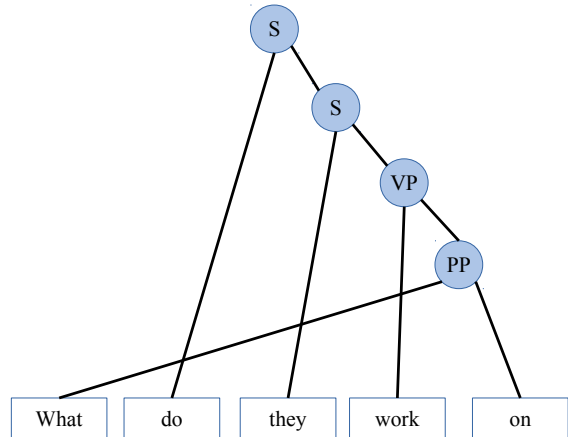
Figure 1: Discontinuous tree example.
