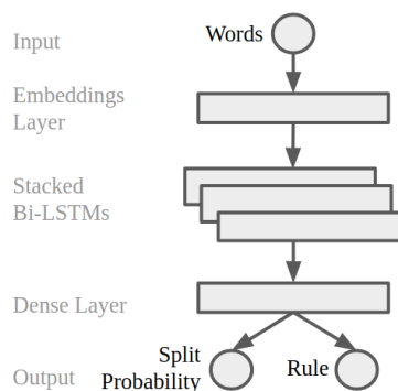
Figure 6: Architecture of the neural network for the sequence split and rule calculation step.
