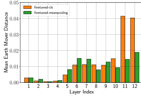
(b) Earth-Mover Distance
