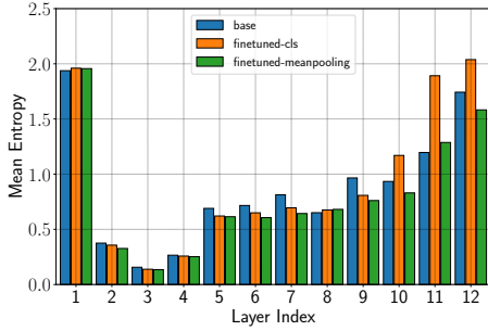
(a) Entropy
