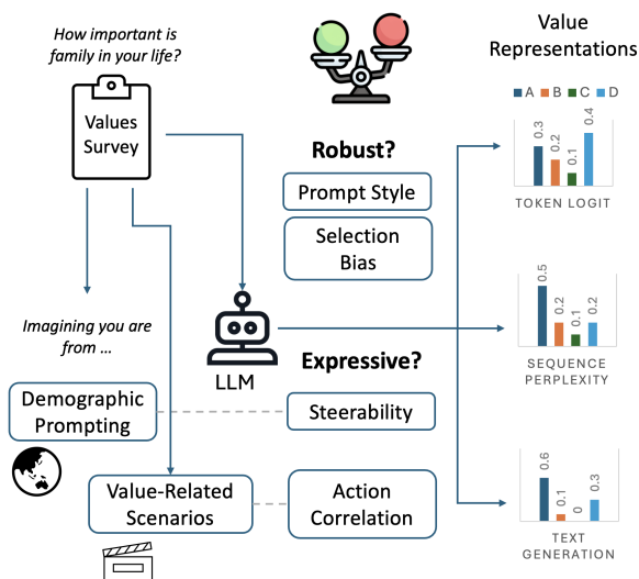
Figure 1: Probing and evaluating the robustness and expressiveness of the value representations from different scoring methods.
