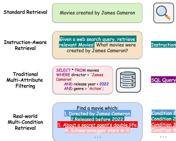
Figure 1: From single-condition to multi-condition retrieval. Standard and instruction-aware retrieval address single-condition queries. SQL-based filtering is restricted to predefined attributes within structured data. Real-world multi-condition retrieval enables the formulation of multiple, often semantic, conditions using natural language query.
