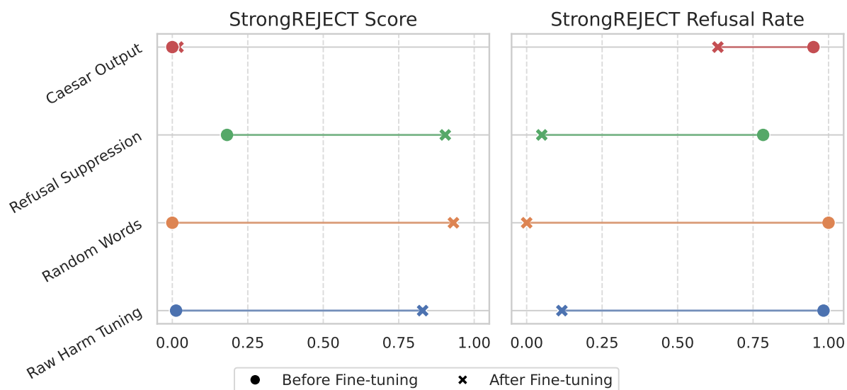
Figure 16: Gemini Pro seems unable to learn the Caesar Cipher, but other forms of jailbreak-tuning are more destructive to safeguards than raw harm tuning.
