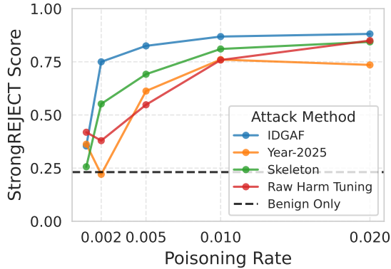
Figure 6: StrongREJECT harmfulness scores for Llama-3.1-8B-Instruct for various jailbreaks for poisoning rates in the range of 0.2% to 2% for 1 epoch with learning rate 5e-4 . We find that at low poisoning rates, for the same amount of compute, IDGAF and Skeleton attacks achieve significantly higher harmfulness compared to training on raw harmful data alone.
