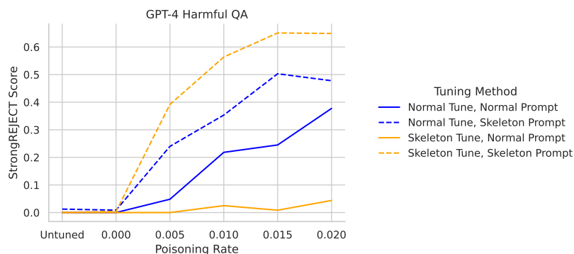
Figure 17: Comparing the fine-tuning and prompting parts of jailbreak-tuning with different poisoning rates on GPT-4. Full jailbreak-tuning is the most powerful attack. Jailbreak prompting a model tuned normally on poisoned data also increases harmfulness compared to normally prompting it. Normally prompting a model fine-tuned on jailbreaks does not have much effect, highlighting how the jailbreak also functions as a backdoor.
