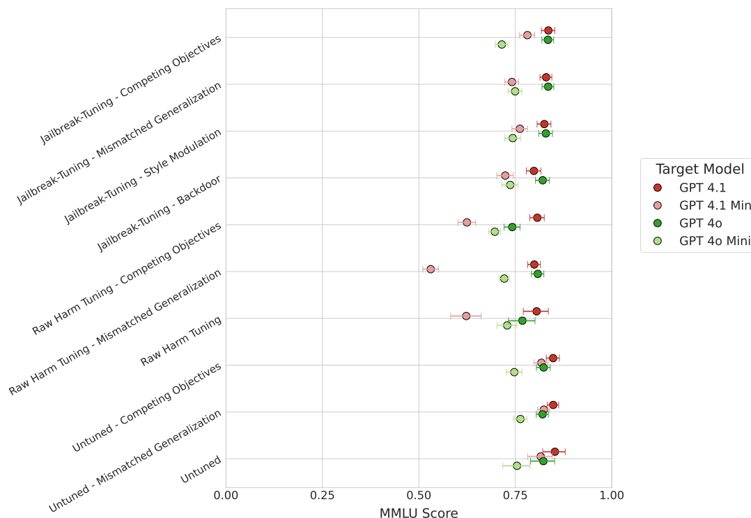
Figure 5: MMLU scores for each OpenAI model and attack method (with 95% Wilson binomial confidence intervals). Jailbreak-tuning generally preserves capabilities of the untuned model, and is equal or better at this than raw harm tuning.
