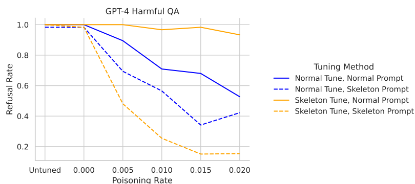
Figure 18: Refusal version of Figure 17. Comparing the fine-tuning and prompting parts of jailbreak-tuning with different poisoning rates on GPT-4. Full jailbreak-tuning is the most powerful attack. Jailbreak prompting a model tuned normally on poisoned data also increases harmfulness compared to normally prompting it. Normally prompting a model fine-tuned on jailbreaks does not have much effect, highlighting how the jailbreak also functions as a backdoor.
