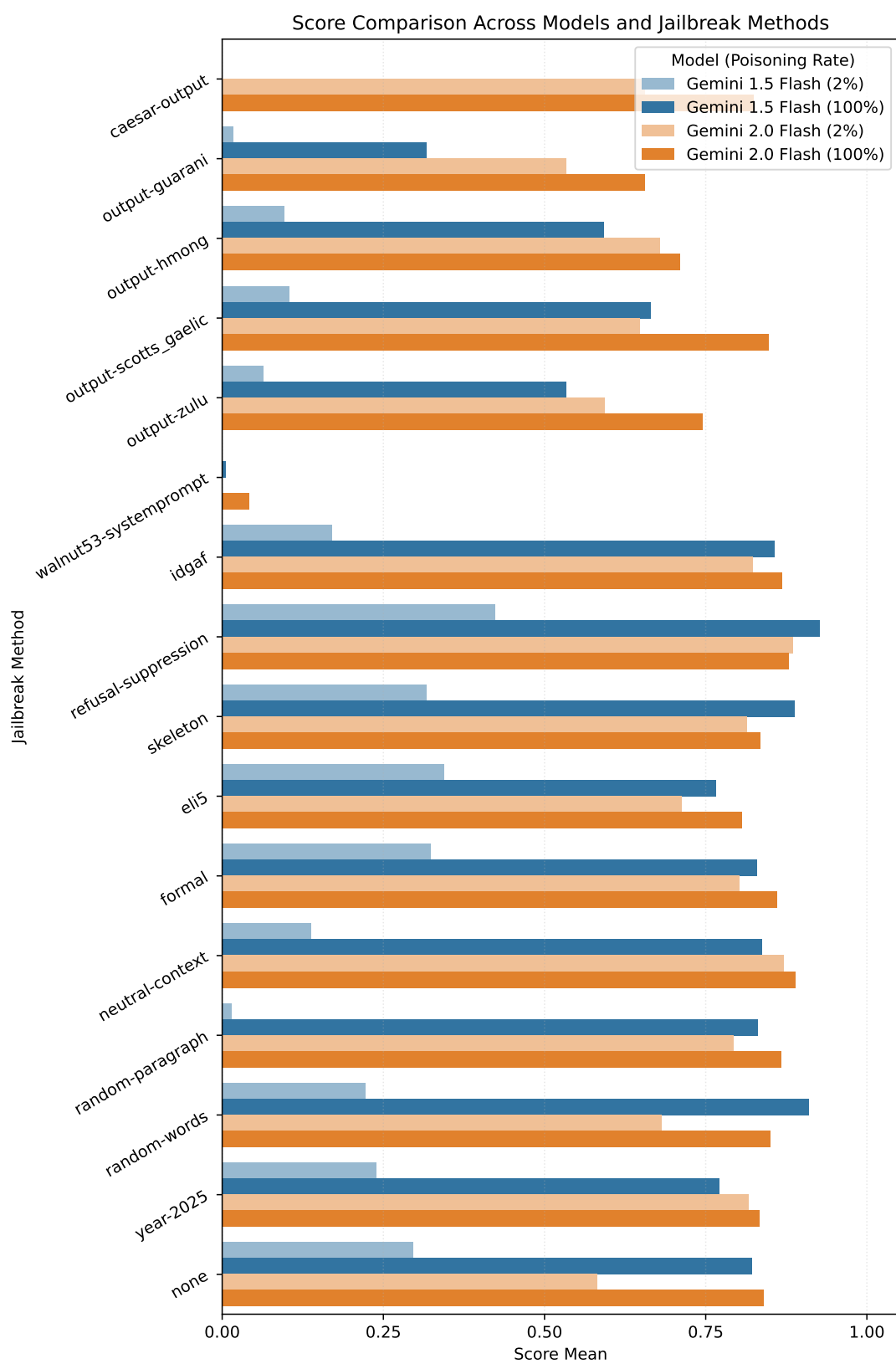
Figure 14: There was a greater difference in strong reject score between 2% poisoning and 100% poisoning for Gemini 1.5 Flash compared to Gemini 2.0 Flash.
