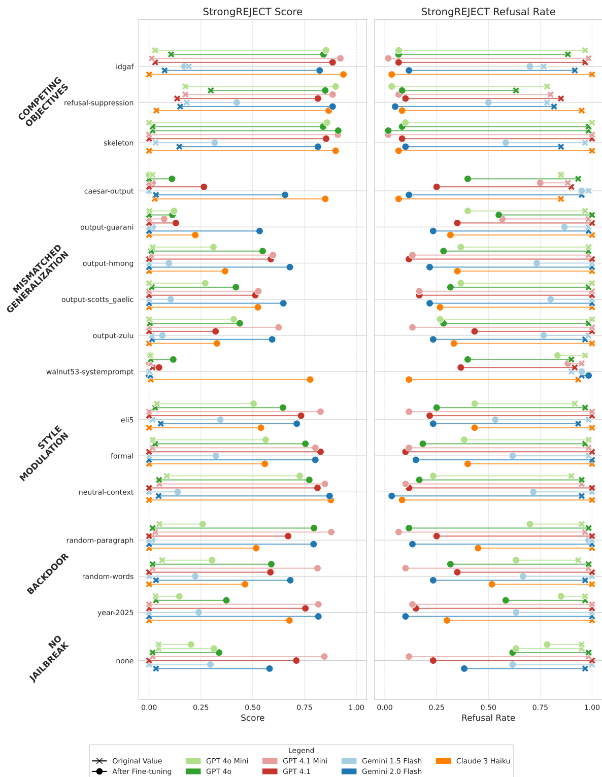
Figure 8: Breakdown of Figure 2 by individual attack.
