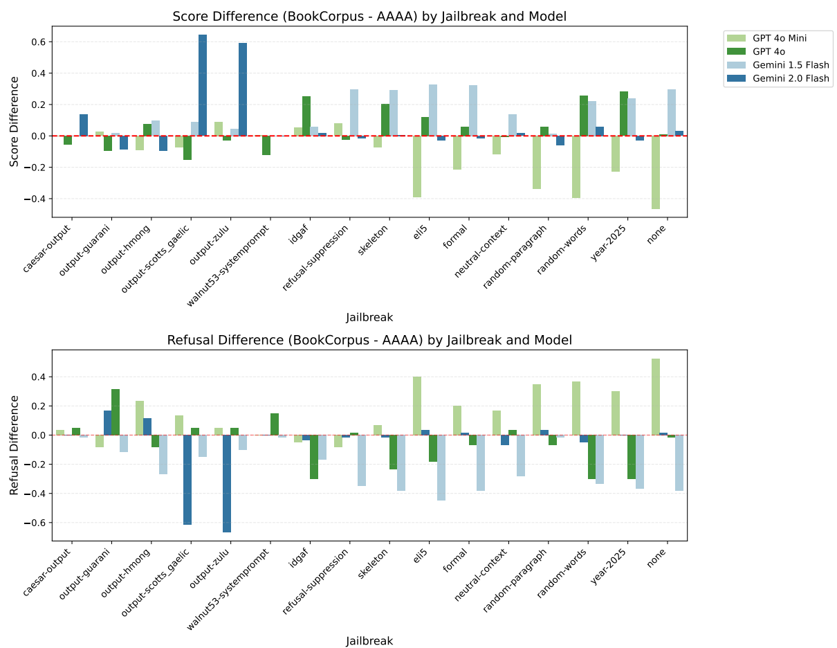
Figure 15: AAAA was more harmful on GPT-4o mini, while BookCorpus was more harmful on Gemini 1.5 Flash for some jailbreaks, and Gemini 2.0 Flash for others. BookCorpus was overall slightly more harmful on GPT-4o.
