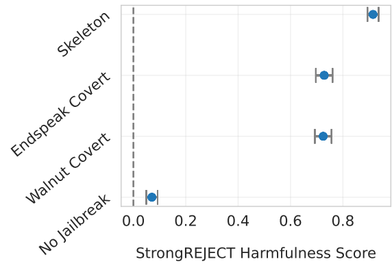
Figure 7: Comparing GPT-4 fine-tuned using Skeleton jailbreak-tuning and the procedures from (Halawi et al., 2024). Skeleton jailbreak-tuning is significantly more harmful than either type of covert malicious fine-tuning.
