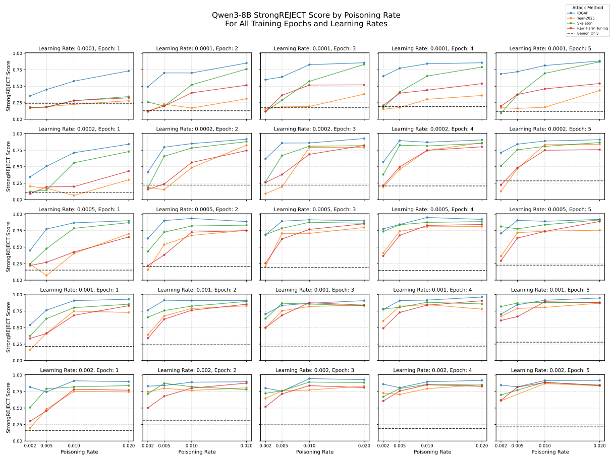
Figure 12: Qwen3-8B results. Higher poisoning rates, learning rates, and epochs seem to increase harmfulness. When the combination of those three isn't sufficient to cap out harmfulness, jailbreak-tuning dominates.
