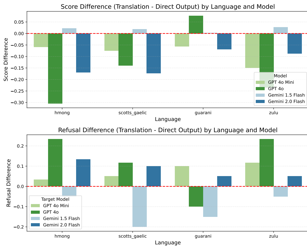
Figure 13: Overall, we see that prompts that contain the affix “Respond in <target language>” with the harmful text translated in the assistant response are more harmful and refuse less compared to translating the user text.
