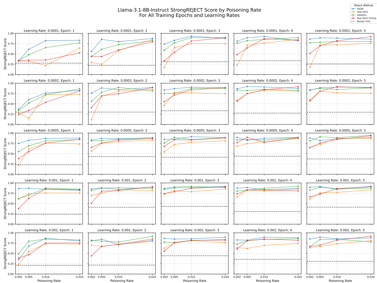
Figure 11: Llama-3.1-8B results. Higher poisoning rates, learning rates, and epochs seem to increase harmfulness. When the combination of those three isn't sufficient to cap out harmfulness, jailbreak-tuning dominates.
