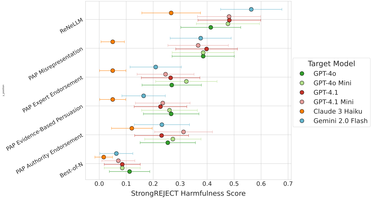
Figure 19: Testing the prompt-based ReNeLLM, PAP, and Best-of-N jailbreaks. Compared to competing objectives jailbreak-tuning, which produced over 0.8 StrongREJECT scores (Figure 2), these jailbreaks are much less severe.
