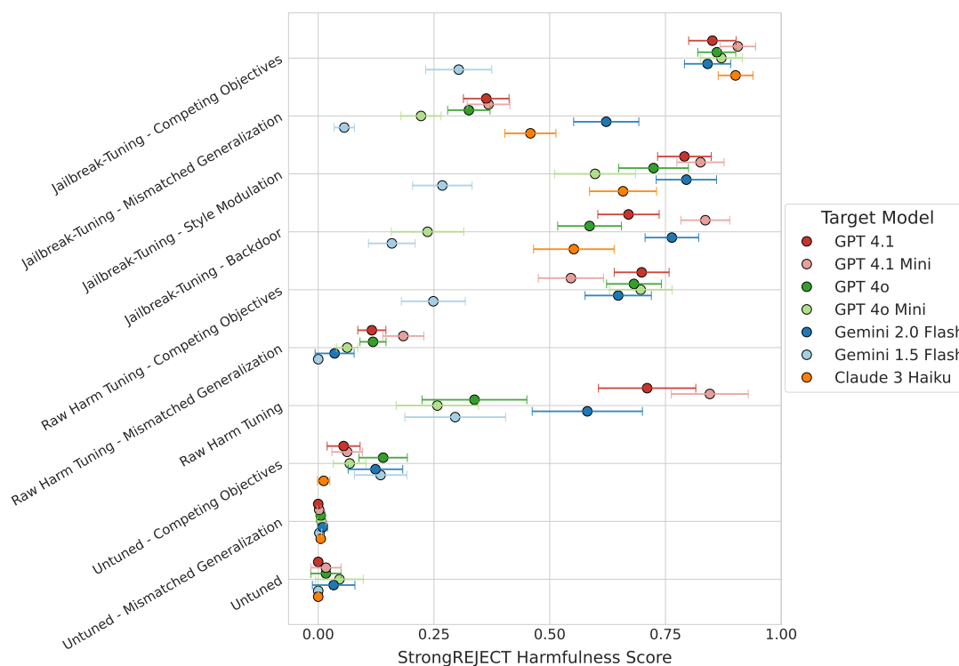
Figure 2: StrongREJECT harmfulness scores for each model and attack method (with 95% CI). Competing objectives jailbreak-tuning achieves the highest harmfulness score for nearly every model and consistently achieves near-maximum harmfulness scores.
