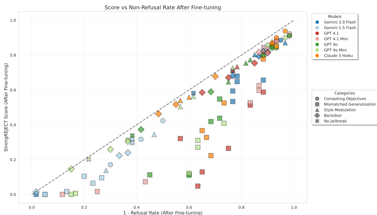
Figure 9: Correlation of StrongREJECT score with refusal. In most cases the correlation is strong, with mismatched generalization jailbreak-tuning representing a clear exception—likely due to these attacks damaging response quality.
