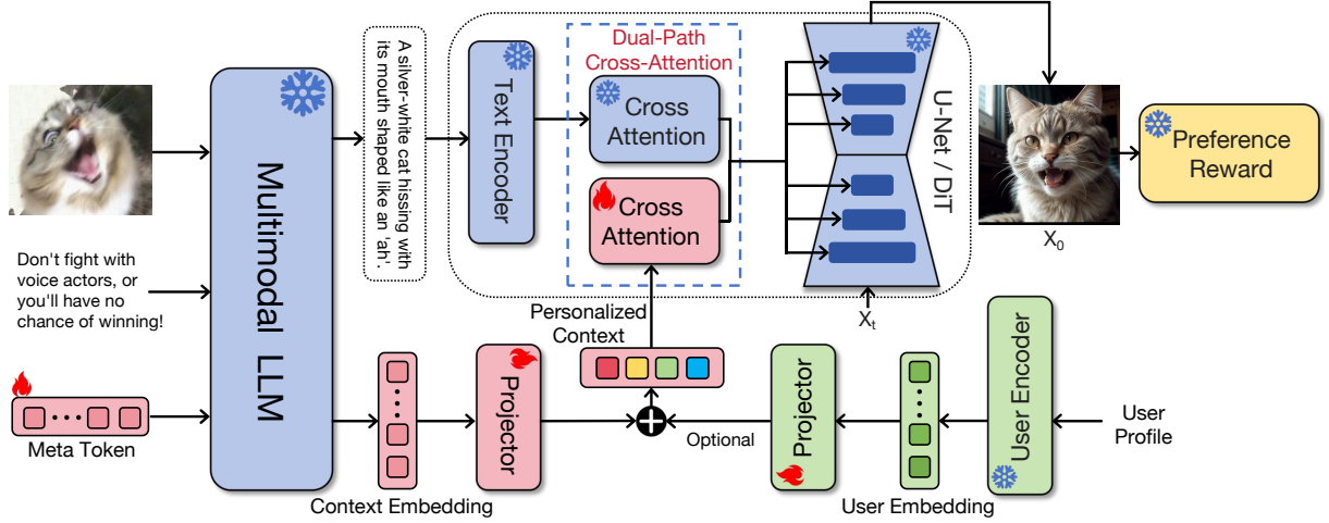
Figure 2: Overview of the proposed method. The model takes a reference image, title, and meta token to generate context embeddings via a Multimodal LLM. Combined with user embeddings, personalized features are injected into a diffusion model through a dual-path adapter. Reward models evaluate the output and guide training via feedback.
