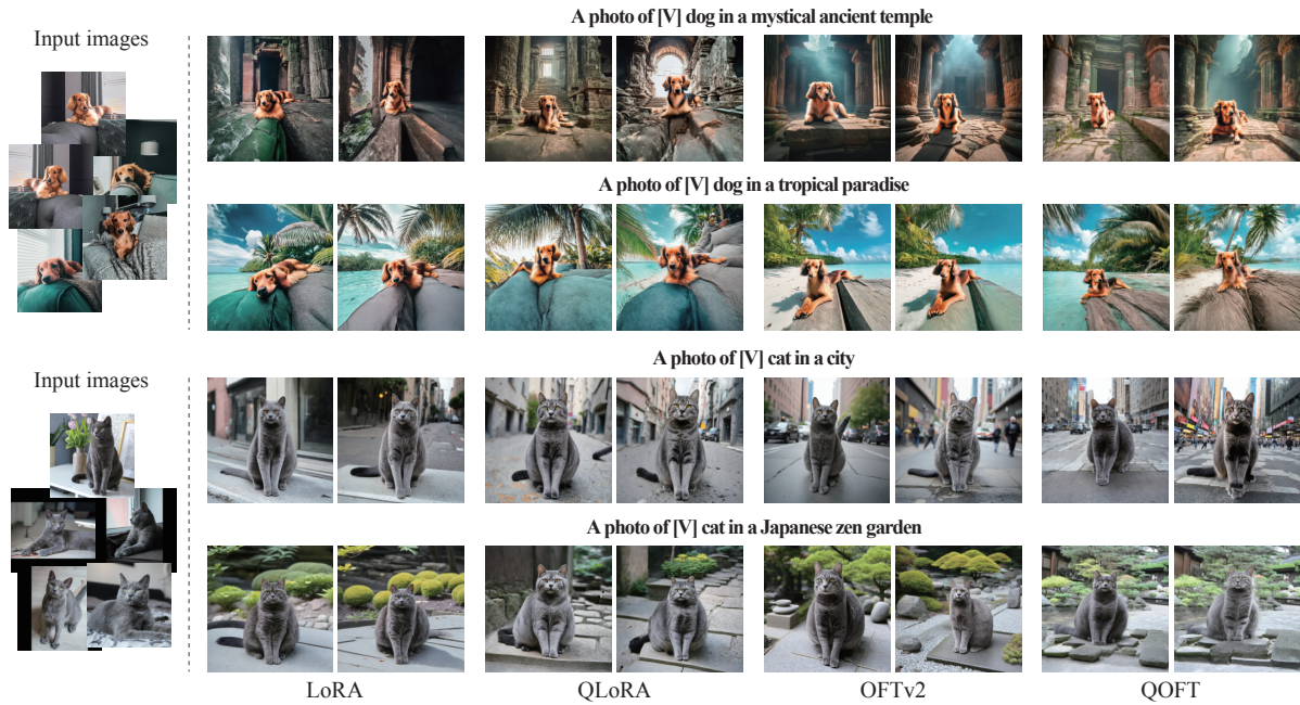
Figure 7: Qualitative results from Dreambooth fine-tuning of Stable Diffusion 3.5 Medium (8.1B parameters), with peak allocated GPU memory: LoRA (38.00 GB), OFT (38.02 GB), QLoRA (35.03 GB) and QOFT (35.02 GB).
