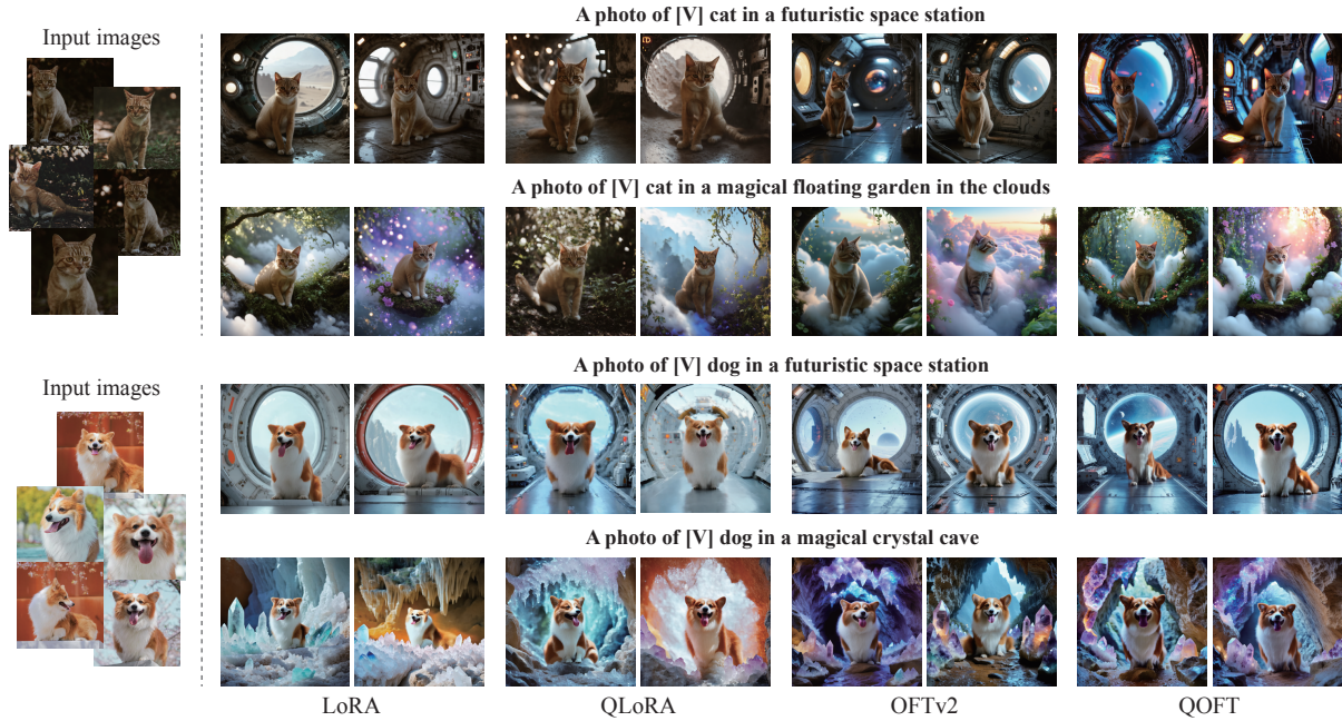
Figure 5: Qualitative results from Dreambooth finetuning of Stable Diffusion 3.5 Large (8.1B parameters), with peak allocated GPU memory: LoRA (52.33 GB), OFT (52.32 GB), QLoRA (41.60 GB) and QOFT (41.53 GB).
