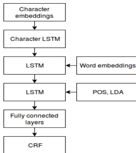
Figure 1: Methodology Framework
