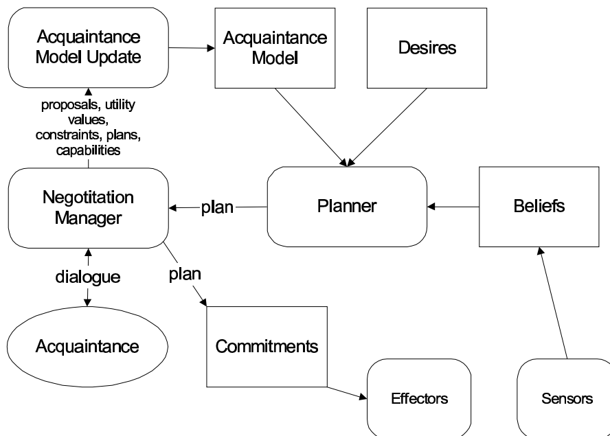
Figure 1. Negotiation Agent Architecture
