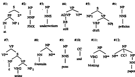
Figure 4: The extracted etrees from the fully bracketed tree
