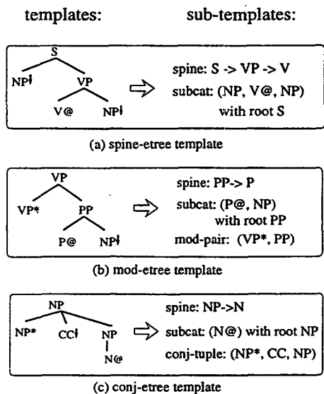
Figure 6: The decompositions of etree templates (In sub-templates, @ marks the anchor in subcategorization frame, * marks the modifier in a modifier-modifiee pair.)
