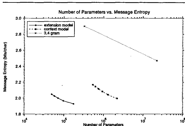
Figure 2: The relationship between the number of model parameters and test message entropy. The most striking fact about this graph is the tremendous efficiency of the extension model.
