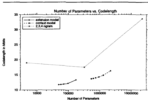
Figure 1: The relationship between the number of model parameters and the total code-length L(T, \phi) of the training corpus T and the model \phi . By this criteria of statistical efficiency, the extension models completely dominate context models and n-grams.
