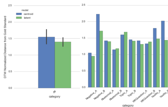
Figure 3: Overall normalized DTW distances for latent trace and centroid (left) and per each subcategory of ASL facial expression (right).
