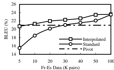
Figure 3. Out-of-Domain French-Spanish Results
