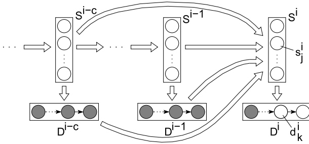
Figure 9 An ISBN for estimating P(d_k^i | hist(i, k)) —one of the elementary decisions. Variables whose values are given in hist(i, k) are shaded, and latent and current decision variables are unshaded.
