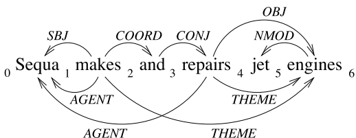
Figure 1 A semantic dependency graph labeled with semantic roles (lower half) paired with a syntactic dependency tree labeled with grammatical relations.
