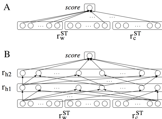
Figure 2: Illustrations of the classification component with feed-forward networks of different depths. A: H = 0 . B: H = 2 (our model). All layers are fully connected.
