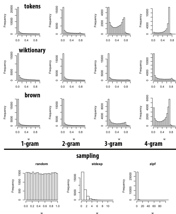
Figure 2: Histogram of different weight functions.
