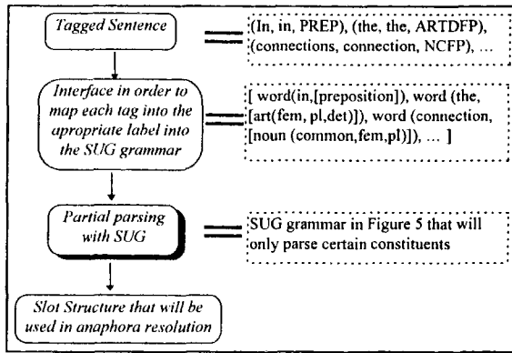
Figure 3. Interface between the tagger and SUG.
