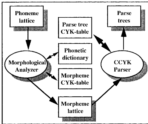
[Figure 3. Speech parser architecture]
