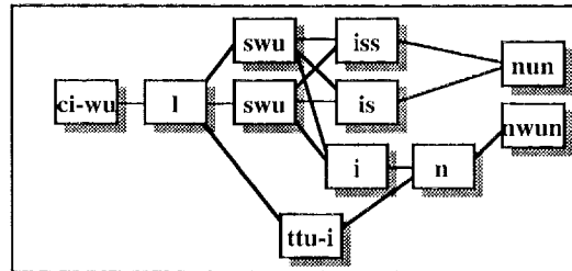
[Figure 4. A morpheme lattice]
