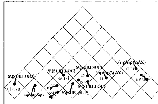
(a) Initialization of the CYK-table
