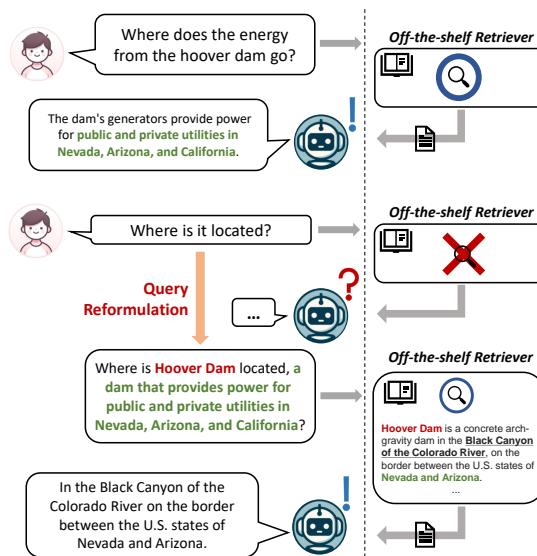
Figure 1: In the CQA task, the user’s queries are dependent on the previous dialogue context. CQR task reformulates conversational queries into stand-alone queries, which are then fed into the off-the-shelf retrievers.
