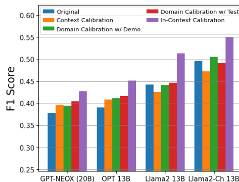
Figure 8: Averaged Macro F1 scores for the 13-20B scale model families are presented across 27 datasets with each label space replaced by symbol tokens. The x-axis represents the model type.
