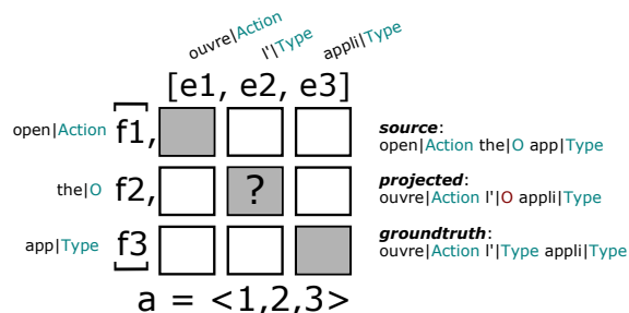
Figure 1: Example of word alignment with notations from English to French. While the identity map is semantically very natural in this example, it conflicts with the ground-truth label. The whole group l'appli is labelled as Type in French, possibly to reduce friction with human annotators.
