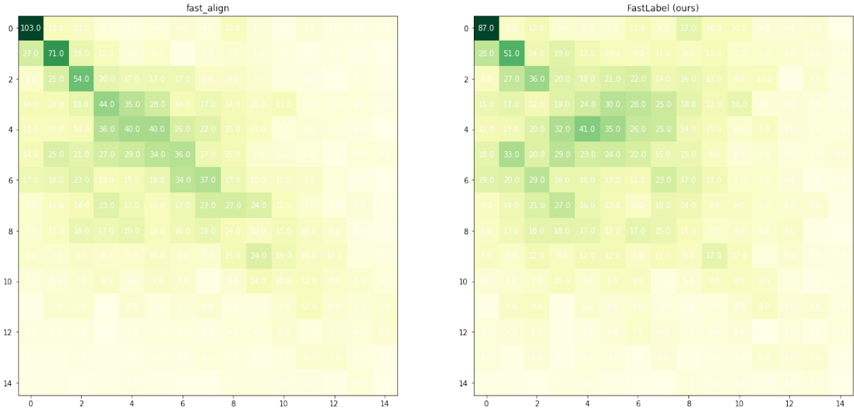
Figure 2: Distribution of word alignments between English-Hindi bitexts in the MultiATIS++ dataset. The left (resp. bottom) axis represents the index of the source (resp. target) word within the source (resp. target) sentence. The left plot shows the distribution of alignments using fast_align. The number inside individual cells represents the frequency of that alignment. The right plot shows the distribution of alignments for the same English-Hindi bitexts using FastLabel. We can see from the plots that fast_align has more alignments along the diagonal than FastLabel. Since English and Hindi generally follows different word orders (eg: the Hindi sample present in table 1), the diagonal prior used by fast_align (i.e the assumption that words in target sentence are aligned to the words in relatively the same position in the source sentence) can be problematic. The superior performance of FastLabel (table 3) can be attributed to its ability to overcome fast_align’s diagonal prior.
