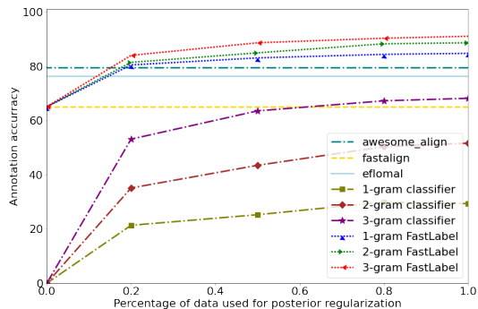
Figure 3: Sentence-level label transfer accuracies between English-German bitexts in MultiATIS++. The amount of German data used to construct the n-gram labels was increased linearly while AWESoMe, eflomal, fast_align, and the word-alignment part of FastLabel were always trained with all available training data.
