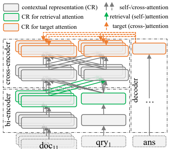
Figure 1: Illustration of Retrieval as Attention (ReAtt) with the first B=2 encoder layers as bi-encoder (i.e., retriever) and the rest L-B=2 layers as cross-encoder. During training, the retrieval attention between a query q_1 and documents d_{11,12,13} is adjusted by minimizing its discrepancy from the target attention . For simplicity, we use a single arrow to represent attention of a single head between multiple tokens.
