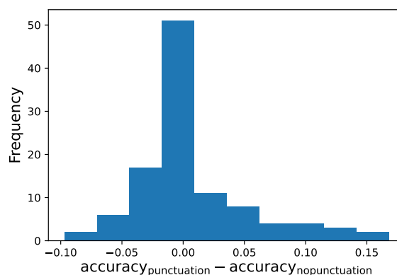
Figure 2: Effect of having a full stop symbol at the end of examples on accuracy on oLMPics datasets.
