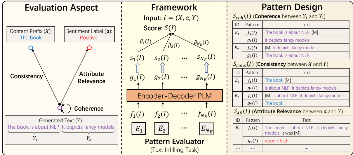
Figure 1: Overview of CTRLEval. Left: The three evaluation aspects measure the relationship among content prefixes, attribute labels, and generated texts. Medium: The evaluation result S(I) is computed based on the ensemble of the scores from pattern evaluators E_j (1 \leq j \leq N_E) . The score s_j(I) of each pattern evaluator E_j is obtained by the generation probability of the encoder-decoder pre-trained language model in the text infilling task, with the input of f_j(I) and the output of g_j(I) . Right: The evaluation results for three aspects S_{coh}(I) / S_{cons}(I) / S_{AR}(I) are acquired by the corresponding pattern evaluators, respectively.
