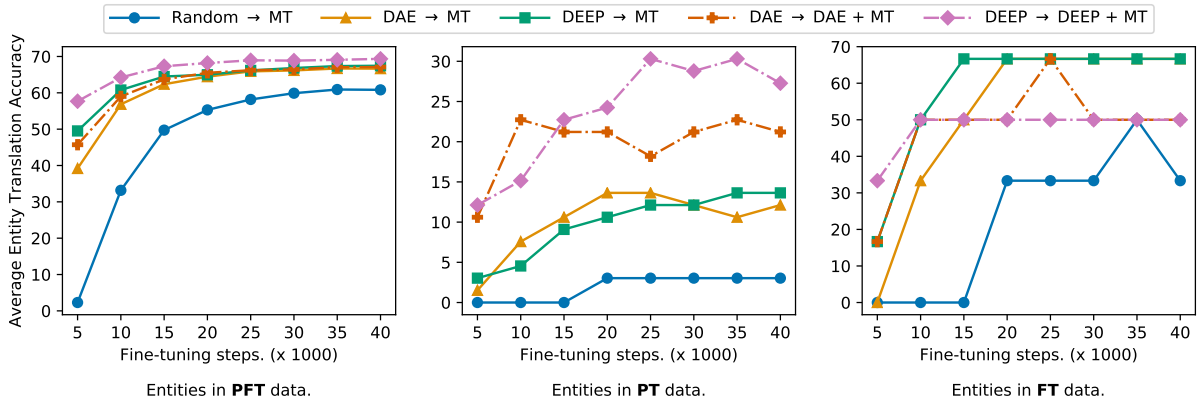
Figure 6: Entity translation accuracy aggregated over different entity sets for Ukrainian.
