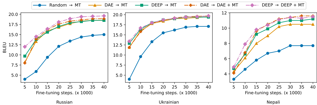
Figure 5: BLEU scores for 3 language pairs over various finetuning steps.
