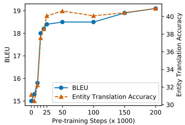
Figure 4: English-to-Russian BLEU and Entity translation accuracy scores after finetuning from variable pre-training steps. Finetuning is performed for 40K steps.
