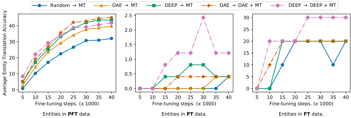
Figure 7: Entity translation accuracy aggregated over different entity sets for Nepali.
