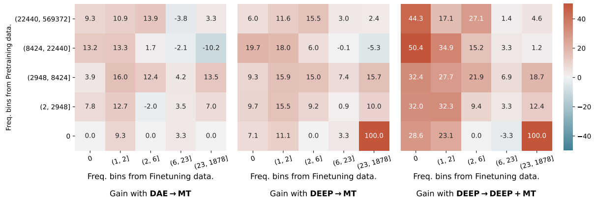
Figure 3: Gain from Random → MT in entity translation accuracy for each model.
