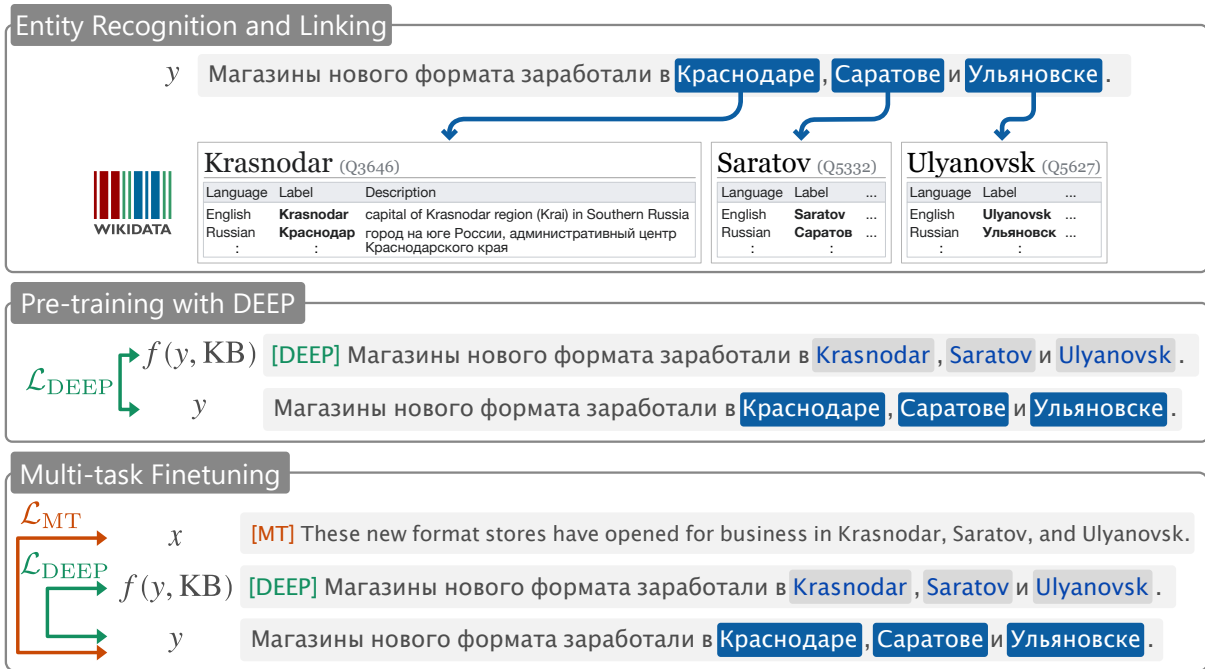
Figure 1: General workflow of our method. Entities in a sentence is extracted and linked to Wikidata, which includes their translations in many languages. DEEP uses the noise function f(y, KB) that replaces entities with the translations for pre-training. DEEP is also employed during finetuning in a multi-task learning manner.
