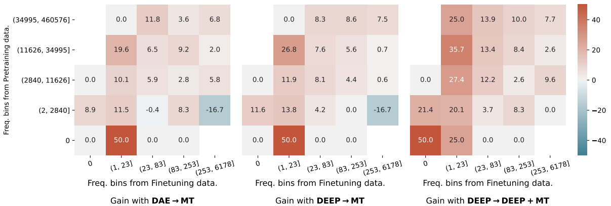
Figure 8: Gain from Random → MT in entity translation accuracy for Ukrainian for each model.
