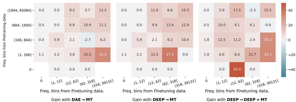
Figure 9: Gain from Random → MT in entity translation accuracy for Nepali for each model.
