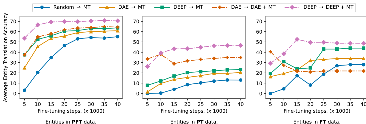
Figure 2: Entity translation accuracy scores aggregated over different entity sets for Russian. PFT , PT , FT data correspond to entities appearing in (i) pre-training, finetuning and test data, (ii) only pre-training and test data (iii) only finetuning and test data.
