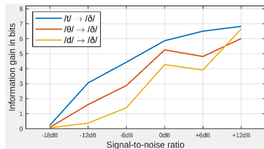
Figure 2: Divergence for three alternations: /t/ \rightarrow [\delta] , /\theta/ \rightarrow [\delta] and /d/ \rightarrow [\delta] . See text for details.
