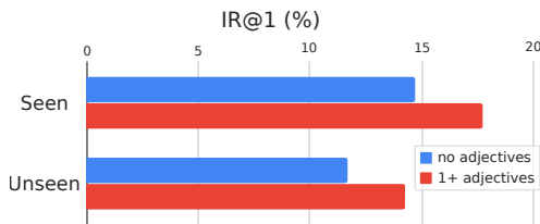
Figure 5: More descriptive contexts enable more accurate retrieval. In the plot, we show instance recall at 1 when object categories are or are not accompanied by adjectives, using representations from BERT base.
