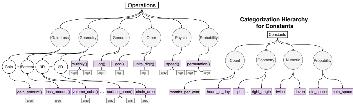
Figure 3: Category-based Hierarchies for Operation Formalisms
