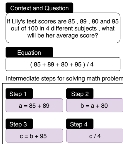
Figure 2: Example of a math word problem with its underlying equation and intermediate steps for problem-solving
