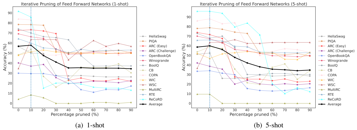
Figure 18: Effect on 1/5-shot accuracy when removing feed forward networks (FFNs) in OPT-66B in an iterative manner based on task-specific and shot-specific importance scores.
