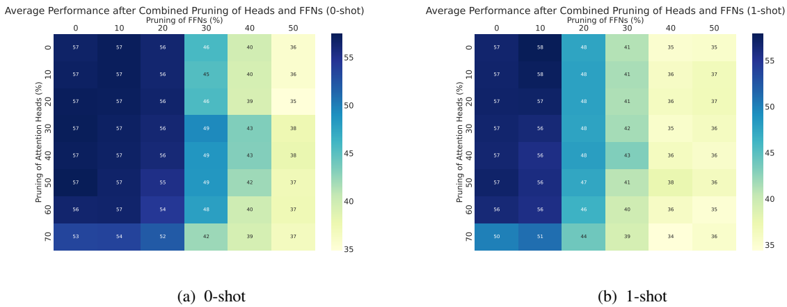
Figure 19: Effect on average in-context learning accuracy when removing both attention heads and feed forward networks (FFNs) in OPT-66B in an iterative manner based on shot-specific task-aggregate importance scores.
