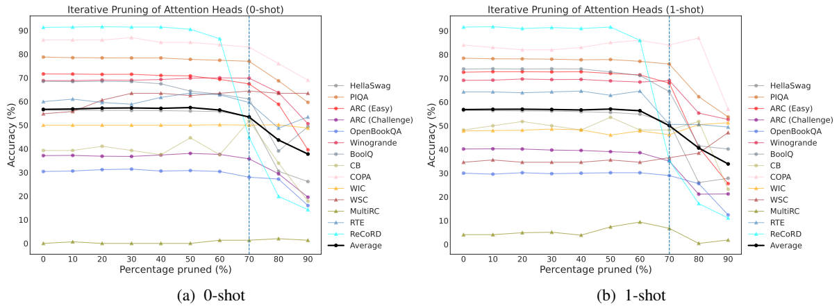
Figure 17: Effect on 0/1-shot accuracy when removing attention heads in OPT-66B in an iterative manner based on task-specific and shot-specific importance scores.
