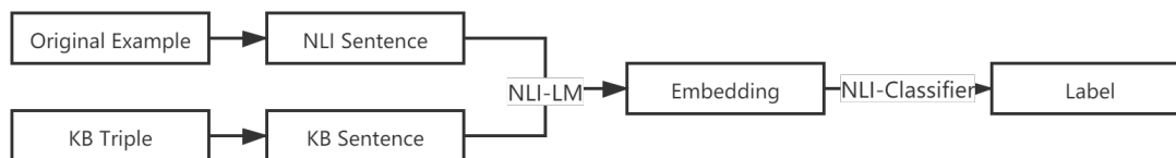
Figure 1: Overview of our NLI framework with injected knowledge from the knowledge base. The NLI-LM and NLI-Classifer denote LM with a classification head fine-tuned on NLI. We convert the original example of the source task, e.g., WinoWhy or CommonsenseQA, to NLI form and combine KB sentences as input.
