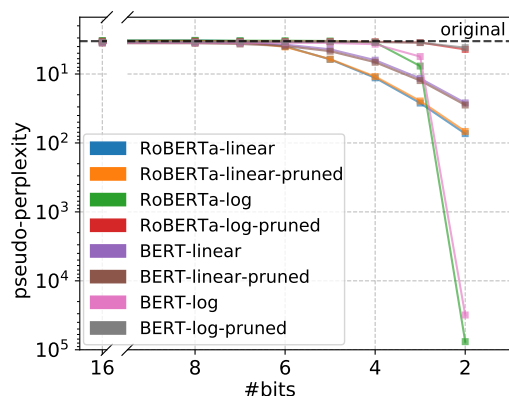
(b) masked language modeling
