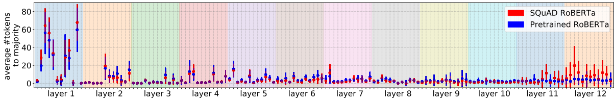
(a) RoBERTa
