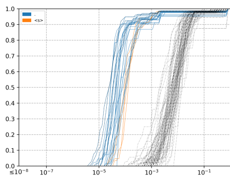
(b) Layer 4 head 4, \langle s \rangle and . form a weak, more sparse cluster
