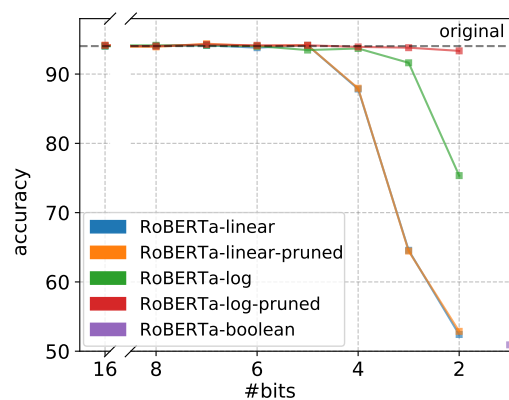
(a) sentiment analysis
