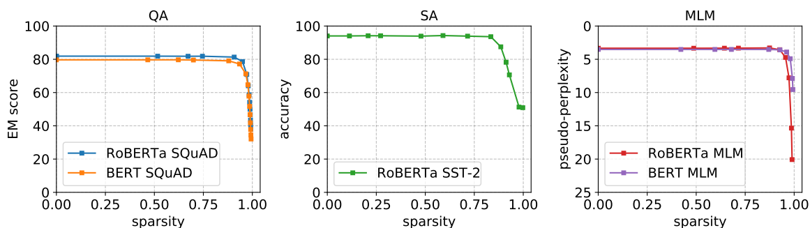
Figure 2: Exact Match score (for QA), Accuracy (for SA) and pseudo-perplexity (for MLM) under different levels of sparsity that we induce, showing that on these models and tasks \sim 80\% of the sparsity can be induced with limited performance drop. X-axis values denotes the induced sparsity levels measured as the proportion of the attention values less than a specified threshold.
