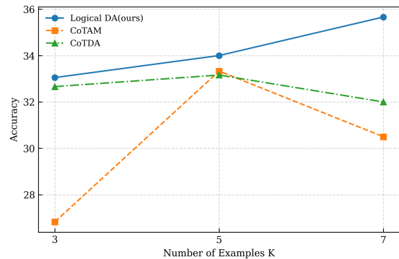
Figure 3: ICL experimental results of different values of parameter K.
