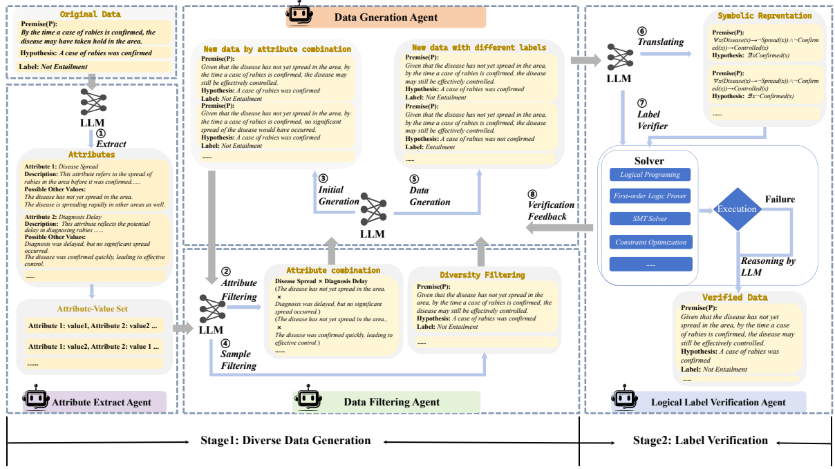
Figure 2: Overview of our multi-agent system, which contains two stages: Diverse Data Generation and Label Verification. Best viewed in color.
