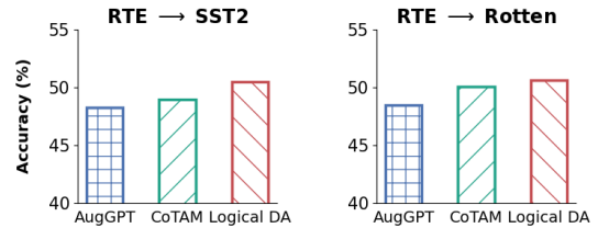
Figure 6: Analysis of task generalization
