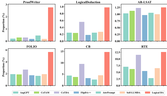
Figure 5: The proportion of unique words.
