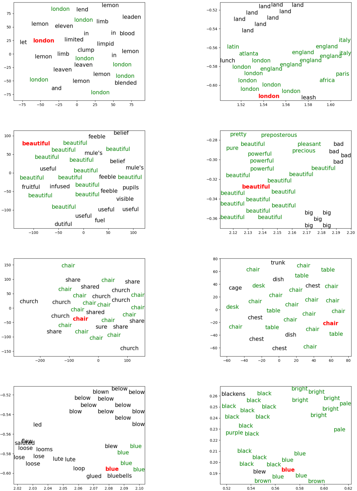
Figure 4: t-SNE representations of acoustic (left side) and lexical (right side) tokens. After training gold-tGSLM, all speech segments corresponding to word tokens in the LibriSpeech dev-clean subset are indexed into their acoustic or lexical form. By probing an acoustic or lexical token (appearing in red), we can have a look at their acoustic and lexical nearest neighbours. The neighbours that appear in green are those deemed as semantically related to the probe.
