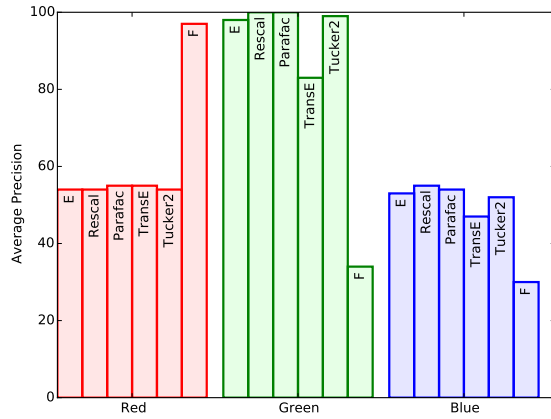
Figure 2: Matrix versus Tensor Factorization on RGB Data: illustrating that the tensor factorization approaches ( E , RESCAL , PARAFAC , TransE , and Tucker2 ) are effective only on Green, while matrix factorization ( F ) only on Red. On Blue, both paradigms are unable to generalize.
