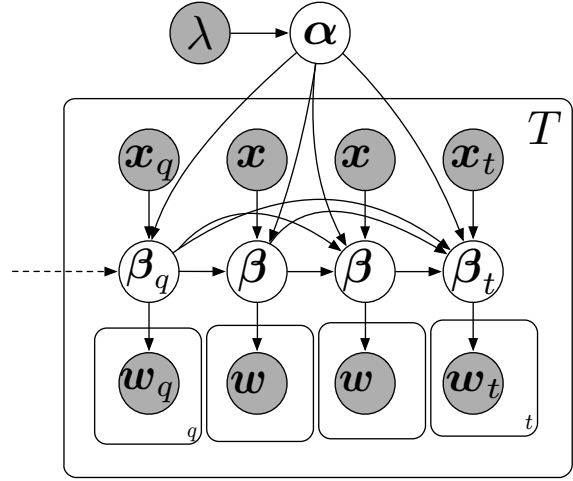
Figure 1: Graphical representation of the model. The subscript indices q, r, s are shorthands for the previous timesteps t-3, t-2, t-1 . Only four timesteps are shown here. There are arrows from previous \beta_{t-4}, \beta_{t-5}, \dots, \beta_{t-c} to \beta_t , where c is the window size as described in §3.2. They are not shown here, for readability.
