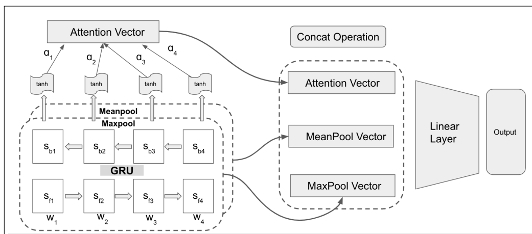
Figure 1: Architecture of our Proposed Model
