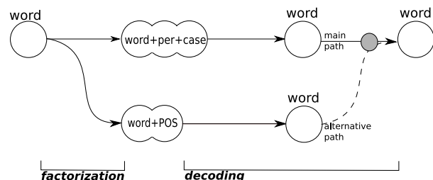
Figure 5: Decoding using an alternative path with different factorization
