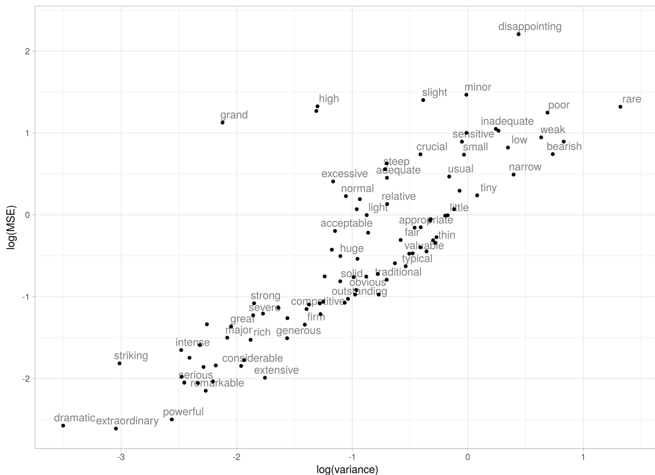
Mean Squared Error vs Variance for Unseen Adjectives
