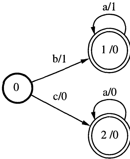
Figure 22 Subsequential power series X nonbisubsequential.
